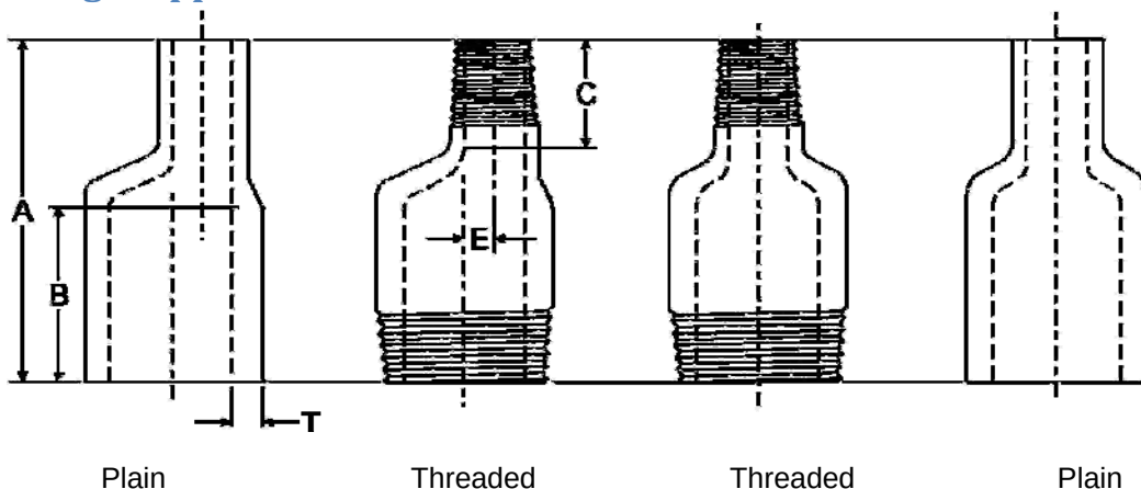
Dimensions of swage nipples (BS 3799:1974)
